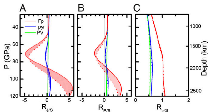
Fig. 3. Pressure dependence of thermally induced heterogeneity ratios (A) R_{\phi/S} = \partial \ln V_{\phi} / \partial \ln V_S , (B) R_{P/S} = \partial \ln V_P / \partial \ln V_S , and (C) R_{\rho/S} = \partial \ln \rho / \partial \ln V_S in Fp, pyrolyte, and perovskitic aggregates along adiabatic (26) (solid line) and superadiabatic (27) (dotted line) mantle geotherms. Aggregates are the same as in Fig. 2.
